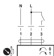
AC 230 V, on-off
