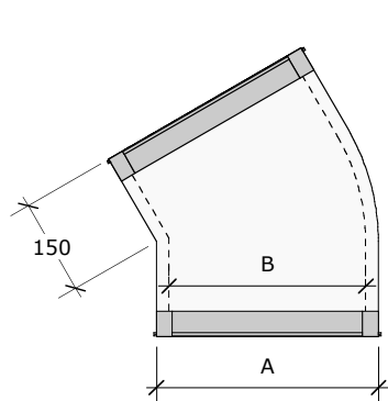
CURVA 30° DB _ _ 30
