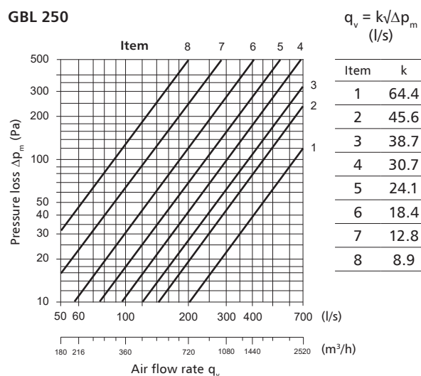
GBL 250
