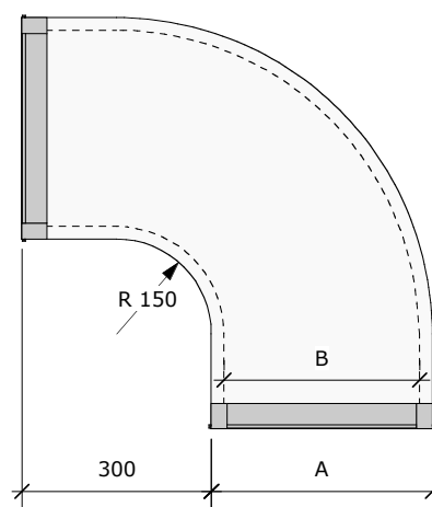
S3 CURVA 90° DB _ _ 90S3
