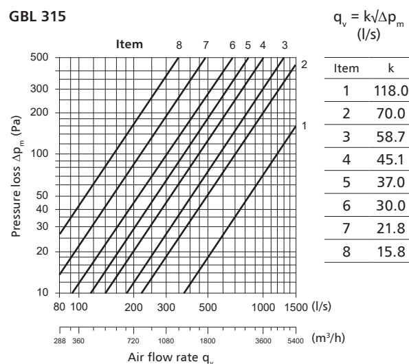
GBL 315
