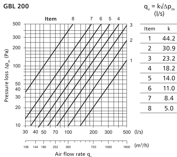
GBL 200
